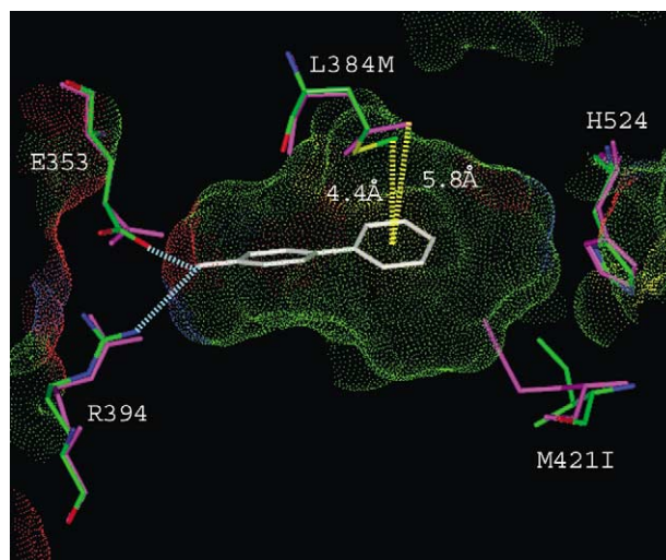
Figure 2. 4-Hydroxy-biphenyl (white), docked to the ER \beta /genistein pocket (colored by atom type), and overlaid with ER \alpha /diethylstilbestrol 7 (magenta). Only key residues, including a Connolly surface of the ER \alpha binding site, are shown for simplicity. The residue numbering scheme for ER \alpha has been used, also for simplicity. Distance monitors show that the biphenyl 'B' ring is in proximity to L384M.
