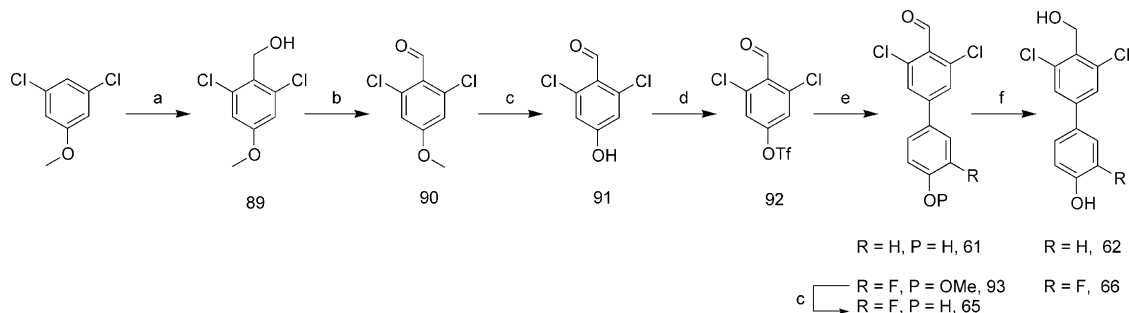
Scheme 6. Reagents and conditions: (a) (1) paraformaldehyde, HCl, \text{H}_2\text{SO}_4 ; (2) \text{NaOH} ; (b) \text{MnO}_2 , \text{C}_6\text{H}_6 ; (c) \text{BBR}_3 , \text{CH}_2\text{Cl}_2 ; (d) \text{TiF}_2\text{O} , \text{C}_6\text{H}_5\text{N} , \text{CH}_2\text{Cl}_2 (e) \text{Pd}(\text{PPh}_3)_4 , \text{Na}_2\text{CO}_3 , DME, \text{H}_2\text{O} , 95^{\circ}\text{C} ; (f) \text{NaBH}_4 , EtOH.
