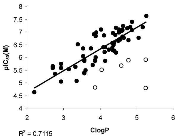
Figure 4. pIC 50 (ER β ) versus ClogP. Compounds in open circles (i.e., 7, 8, 31, 32, 46, and 47) are outliers where detrimental steric factors are significantly influencing affinity.
