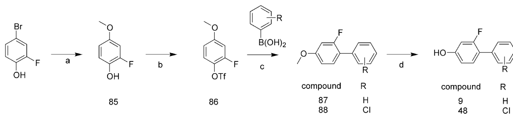
Scheme 5. Reagents and conditions: (a) \text{CuBr} , \text{NaOMe} , DMF; (b) \text{TiF}_2\text{O} , \text{C}_6\text{H}_5\text{N} , \text{CH}_2\text{Cl}_2 (c) \text{Pd}(\text{PPh}_3)_4 , \text{Na}_2\text{CO}_3 , DME, \text{H}_2\text{O} , 95^{\circ}\text{C} ; (d) pyridine hydrochloride, 190^{\circ}\text{C} .
