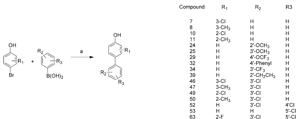
Scheme 2. Reagents and conditions: (a) Pd(PPh 3 ) 4 , Na 2 CO 3 , DME, H 2 O, 95 °C.
