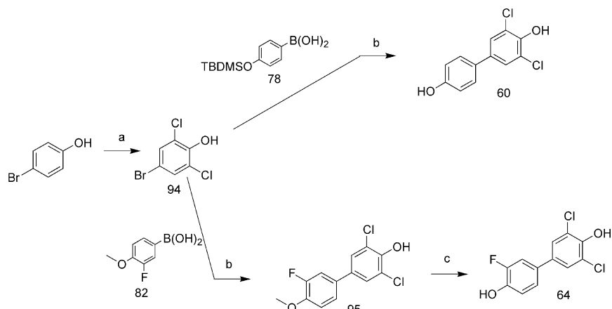
Scheme 7. Reagents and conditions: (a) NCS, CH 3 CN; (b) Pd(PPh 3 ) 4 , Na 2 CO 3 , DME, H 2 O, 95 °C; (c) pyridine hydrochloride, 190 °C.
