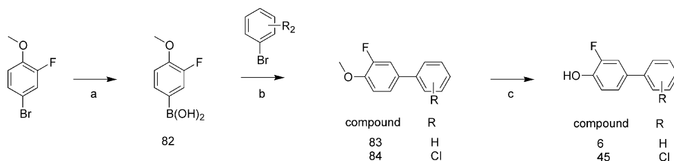
Scheme 4. Reagents and conditions: (a) (1) n -butyllithium, -78^{\circ}\text{C} ; (2) triisopropylborate (3) HCl; (b) \text{Pd}(\text{PPh}_3)_4 , \text{Na}_2\text{CO}_3 , DME, \text{H}_2\text{O} , 95^{\circ}\text{C} ; (c) pyridine hydrochloride, 190^{\circ}\text{C} .
