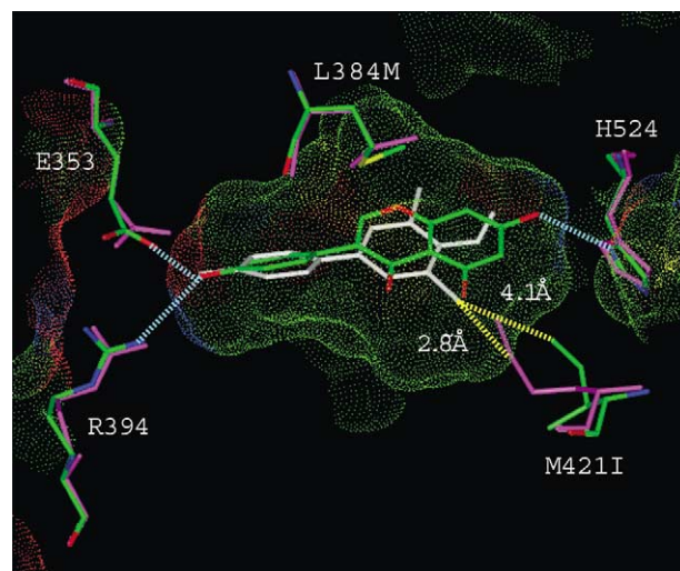
Figure 5. Compound 61 (white), docked to the ER β /genistein pocket (including the ligand and colored by atom type), overlaid with ER \alpha /diethylstilbestrol 7 (magenta). As in Figure 1, only key residues and a Connolly surface of the ER β binding site are shown for simplicity. Again, the residue numbering scheme for ER \alpha has been used. Distance monitors show that the 3'-Cl is in close proximity to M421I.
