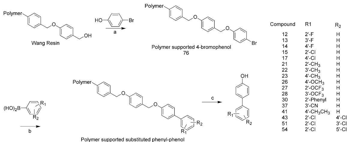
Scheme 1. Reagents and conditions: (a) DIAD, PPh 3 , THF; (b) Pd(PPh 3 ) 4 , Na 2 CO 3 , DME, H 2 O, 80 °C; (c) 50% TFA/CH 2 Cl 2 .
