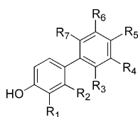
Scheme 7. Reagents and conditions: (a) NCS, CH 3 CN; (b) Pd(PPh 3 ) 4 , Na 2 CO 3 , DME, H 2 O, 95 °C; (c) pyridine hydrochloride, 190 °C.
