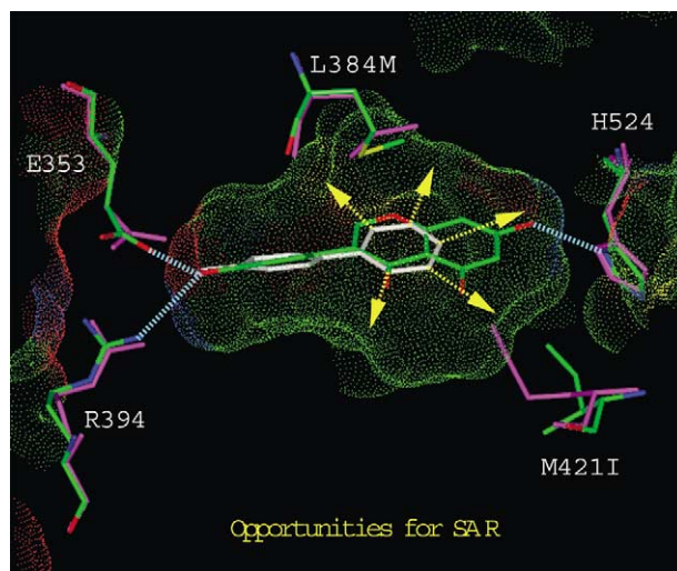
Figure 3. Overlay with genistein ligand included. Arrows indicate opportunities for exploration.
