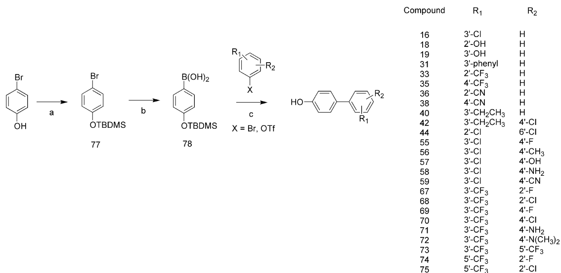
Scheme 3. Reagents and conditions: (a) TBDMS-Cl, imidazole, DMF; (b) (1) n -butyllithium, -78^{\circ}\text{C} ; (2) triisopropyl borate; (3) HCl (c) \text{Pd}(\text{PPh}_3)_4 , \text{Na}_2\text{CO}_3 , DME, \text{H}_2\text{O} , 95^{\circ}\text{C} .
